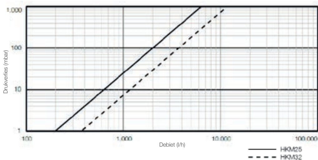
Drukverliescurve HK 25/32
