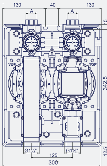
FLOWBOX HK 25/32
