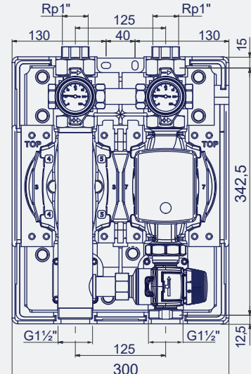
FLOWBOX HKF 25/32
