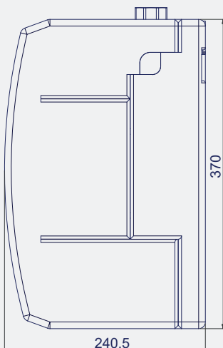
FLOWBOX DN 25/32 Isolatieschaal
