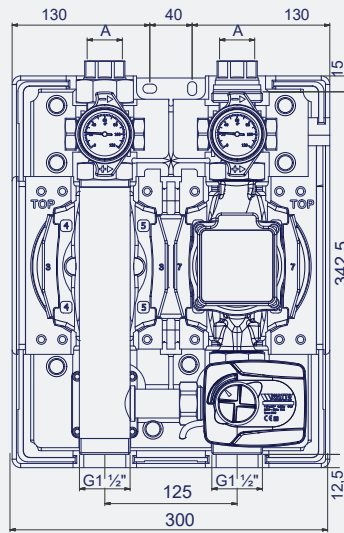
FLOWBOX HKM 25/32
