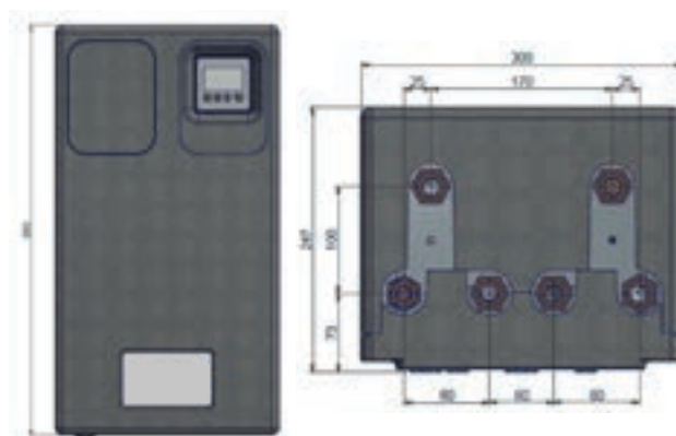
HIU HEAT COMFORT COMPACT E
